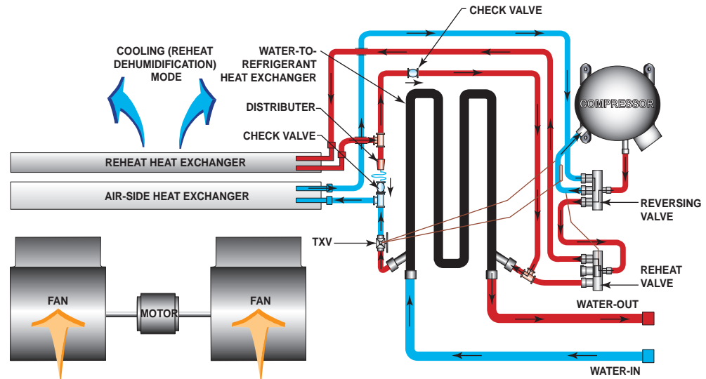
Figure 12. Hot gas reheat
