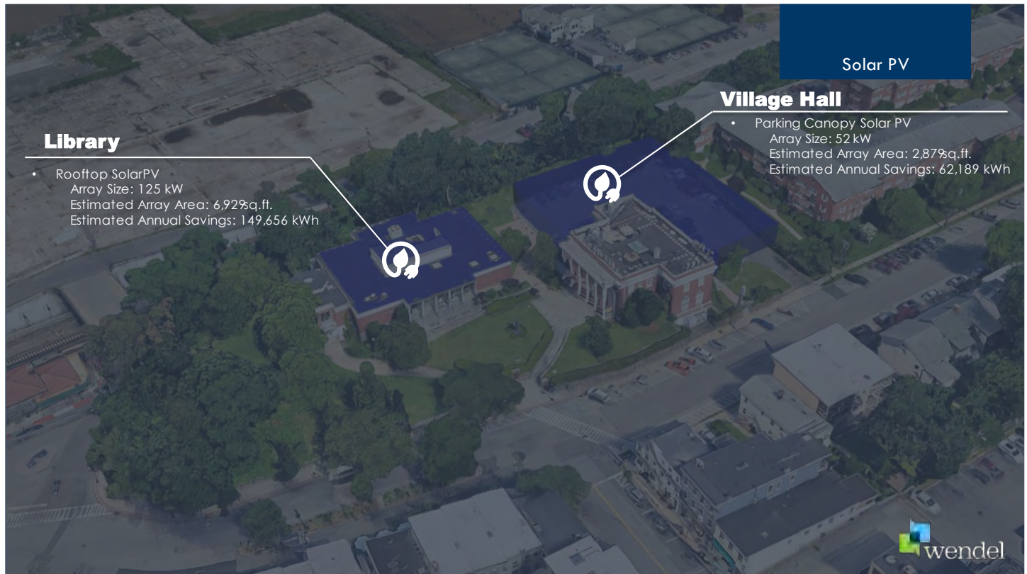
Figure 4. Locations of proposed roof mount and parking canopy solar arrays.
