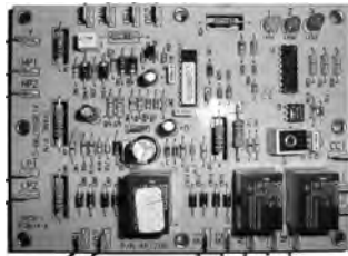
Figure 37. Deluxe 24V control board
