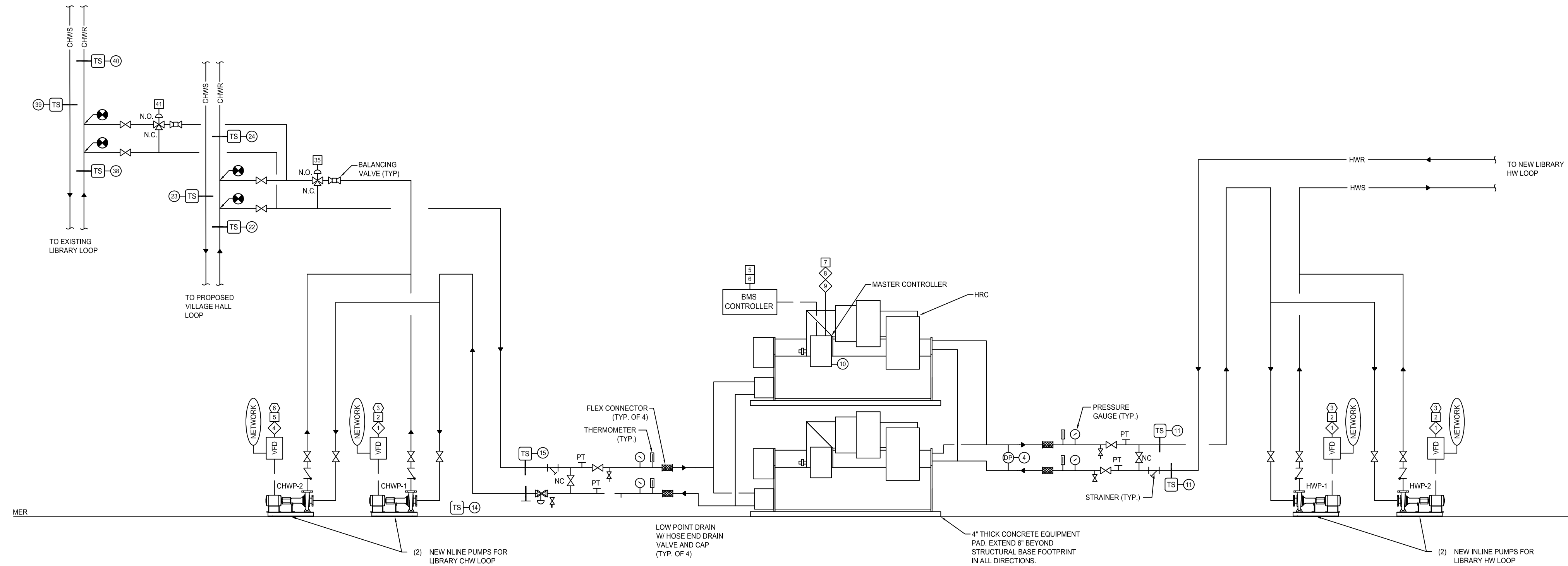
3 VILLAGE OF HASTINGS-ON-HUDSON | LIBRARY AIR SOURCE HEAT PUMP SCHEMATIC (TYP. OF 4) SCALE: NONE
