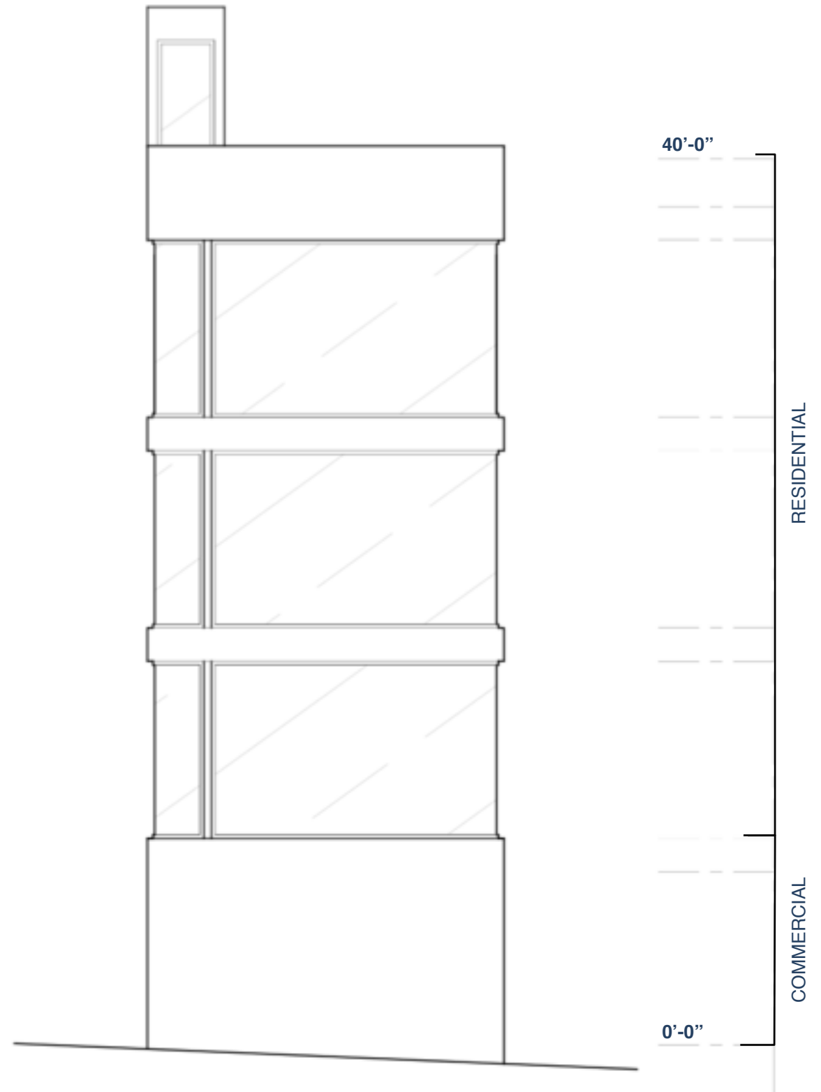
NORTH ELEVATION
